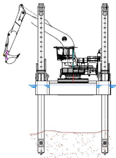
AFT VIEW
